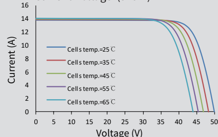
Current-Voltage (545W)
