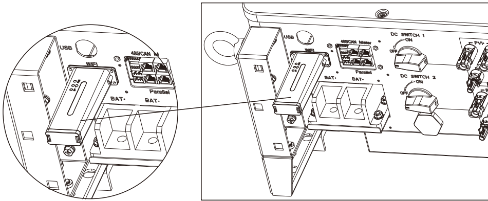
The Wireless Communication Interface Details
